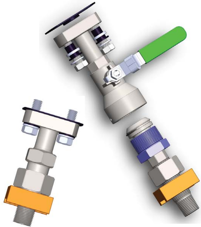
TM-SBVT-AA-Exploded Rendering
