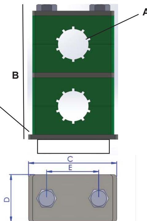
WELD PAD MOUNT
