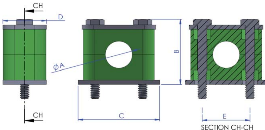
2 STACK TUBING SUPPORT CLAMP (units: inches)
